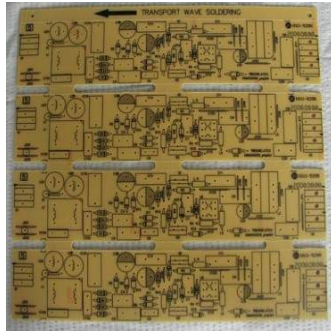
1-Layer PCB material:FR1 Borad thickness:1.2mm copper thickness:1oz panel size: 100.20mm*100.20mm(4pcs)
