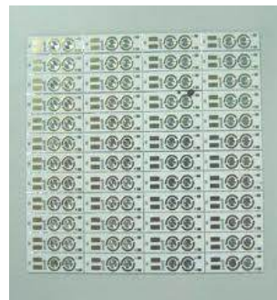
HASL PCBA (LED pcb) material:AL Borad thickness:1.8mm copper thickness:1.5oz size: 140.30mm*140.30mm
