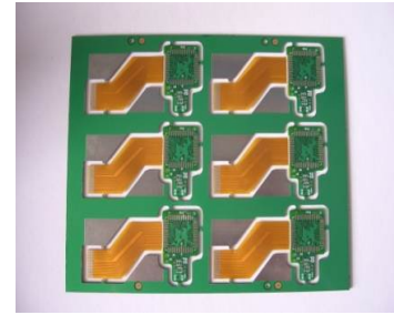
1-Layer Rigid Flex PCB material:FR4, PI Borad thickness:0.8mm copper thickness:1oz panel size: 102.28mm*114.40mm
