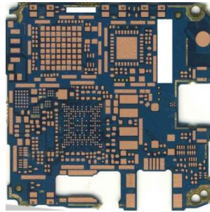
4-Layer ENIG PCB material:FR4 Borad thickness:1.6mm copper thickness:2oz size: 112.60mm*112.60mm
