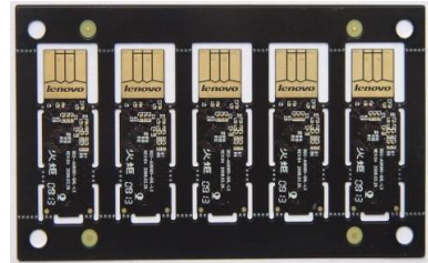
2-Layer gold finger PCB material:FR4 Borad thickness:1.6mm copper thickness:1oz panel size: 226.62mm*92.80mm(5pcs)
