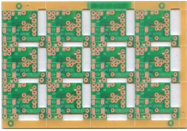
1-Layer OSP PCB material:CEM-3 Borad thickness:1.6mm copper thickness:1oz panel size: 96.66mm*135.20mm(12pcs)
