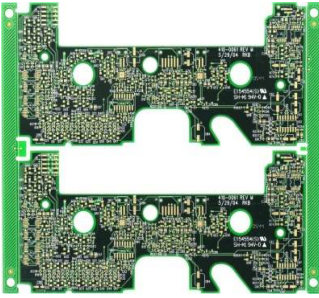
6-Layer ENIG PCB material:FR4 Borad thickness:1.6mm copper thickness:2oz panel size: 142.86mm*120.08mm (2pcs)
