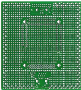
Universal pcb material:FR4 Borad thickness:1.6mm copper thickness:1oz size: 144.52mm*144.52mm
