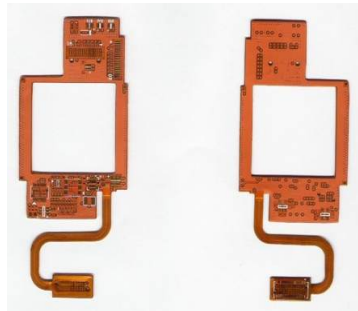
2-Layer FPC material:PI Borad thickness:0.1mm copper thickness:0.5oz size: 82.28mm*34.22mm
