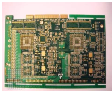
8-Layer gold finger immersion gold PCB material:FR4 Borad thickness:2.0mm copper thickness:4oz size: 216.36mm*152.42mm
