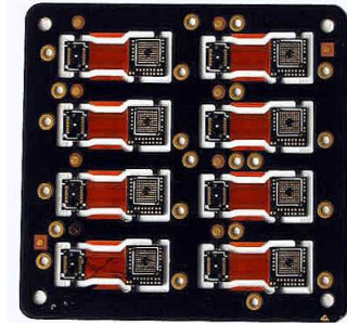
2-Layer Rigid Flex PCB material:FR4, PET Borad thickness:0.8mm copper thickness:1oz panel size: 102.28mm*114.40mm
