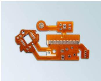
4-Layer FPC material:PET Borad thickness:0.3mm copper thickness:1oz size: 76.28mm*54.24mm
