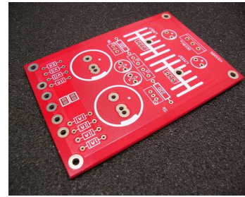
4-Layer HASL PCB material:FR4 TG170 Borad thickness:1.6mm copper thickness:1oz size: 132.66mm*96.54mm
